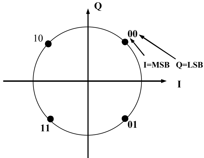
Figure 2.4.10-2: Constellation Mapping
