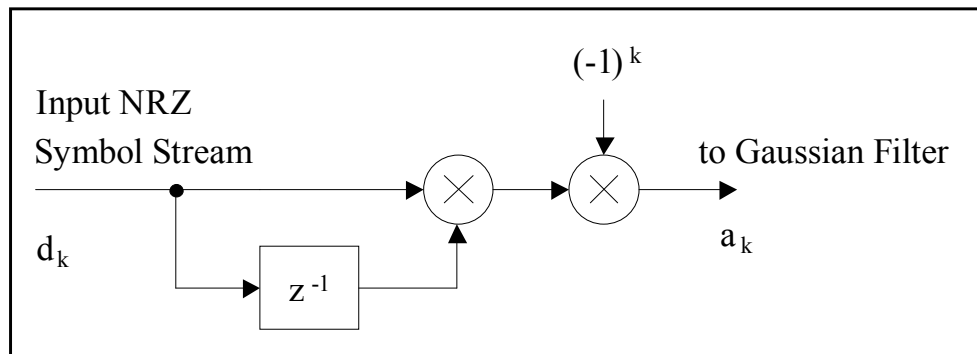
Figure 2.4.22A-2: GMSK Precoder
