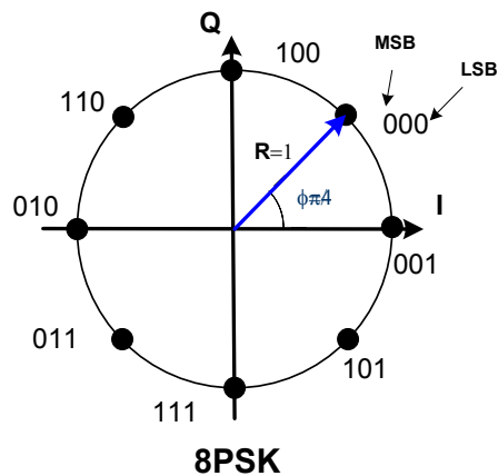
Figure 2.4.23-5: 8PSK Symbol Mapping into Constellation (CCSDS 131.3-B-1 and CCSDS 131.0-B-3)
