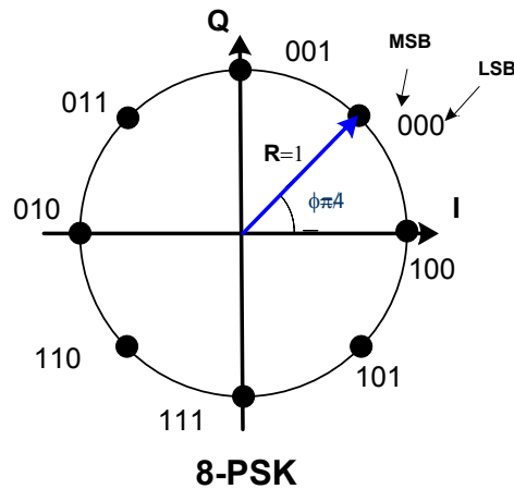
Figure 2.4.18-18: 8PSK Symbol Mapping into Constellation (CCSDS 131.2-B-1)
