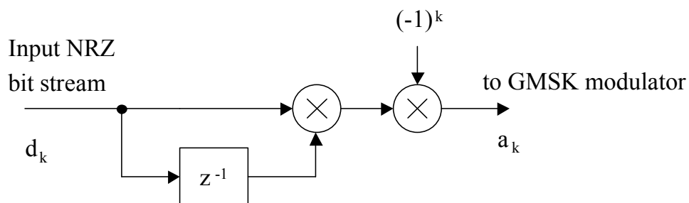
Figure 2.4.17B-1: GMSK Precoder
