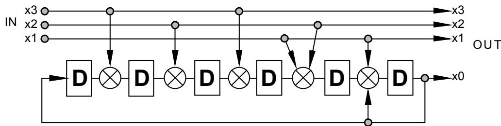
Figure 2.4.18-3: Convolutional Coder Recommended for High Data Rates
