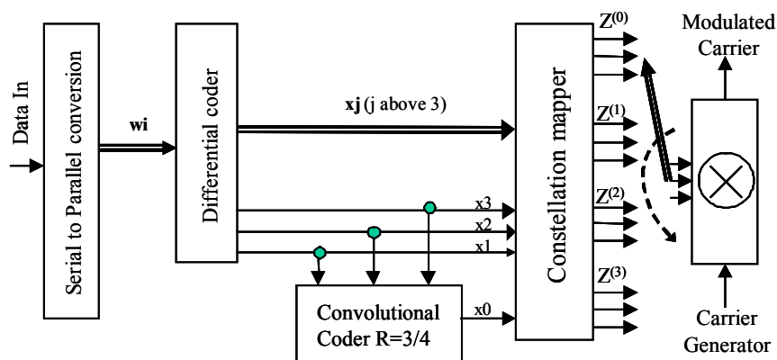
Figure 2.4.18-1: Structure of the 4D 8PSK-TCM Coder/Mapper
