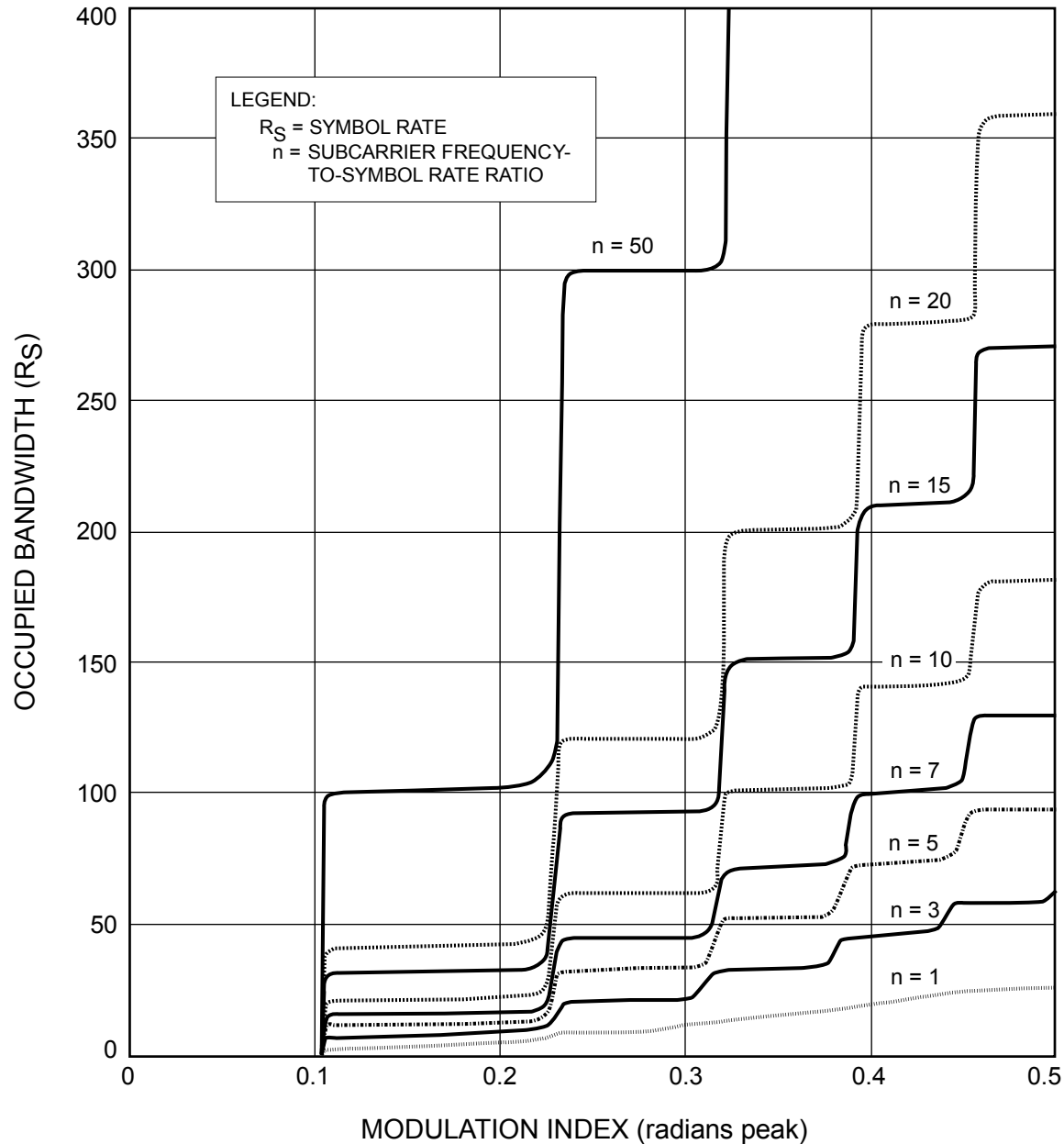
Figure 4.2.3-1: Occupied Bandwidth of Unfiltered PCM/PSK/PM Signal with a Square-Wave Subcarrier
