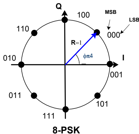
Figure 2.4.18-19: 8PSK Symbol Mapping into Constellation (CCSDS 131.3-B-1 and CCSDS 131.0-B-3)
