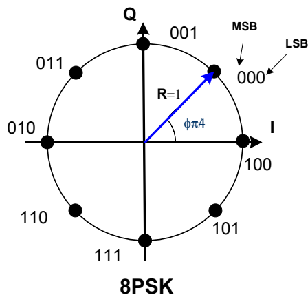
Figure 2.4.23-4: 8PSK Symbol Mapping into Constellation (CCSDS 131.2-B-1)
