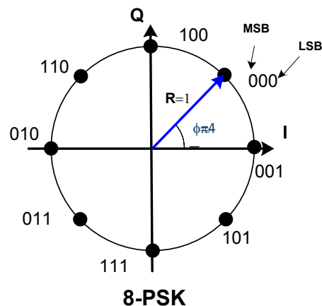
Figure 2.4.17A-5: 8PSK Symbol Mapping into Constellation (CCSDS 131.0-B-3 and CCSDS 131.3-B-1)
