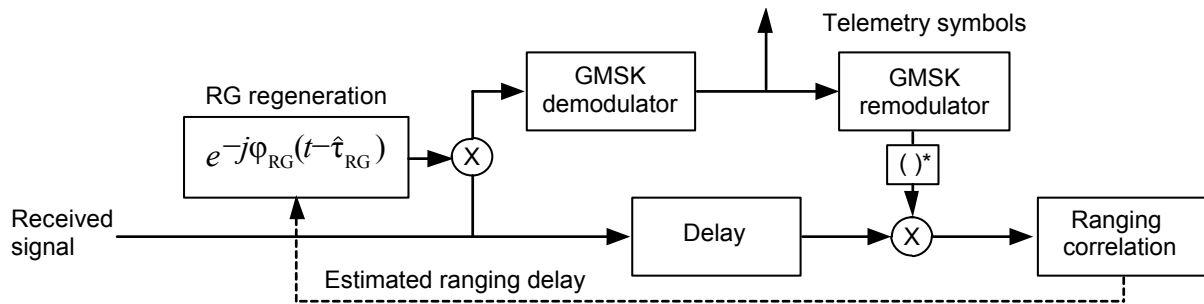
Figure 2.4.22B-3: High-Level Diagram of GMSK+PN RG Receiver with Ranging Cancellation
