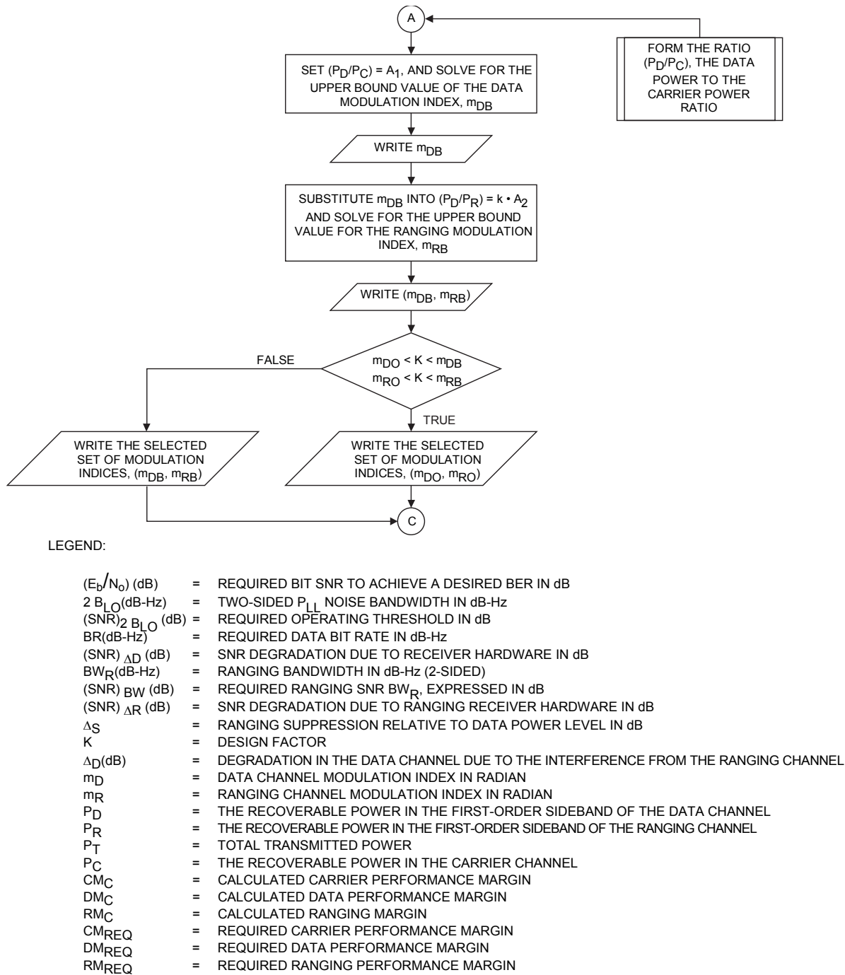
Figure 4.1.1-1: MT's Algorithm: An Algorithm to Search for a Set of Optimum Modulation Indices for Simultaneous Command/Telemetry/Range Operations (Continued)
