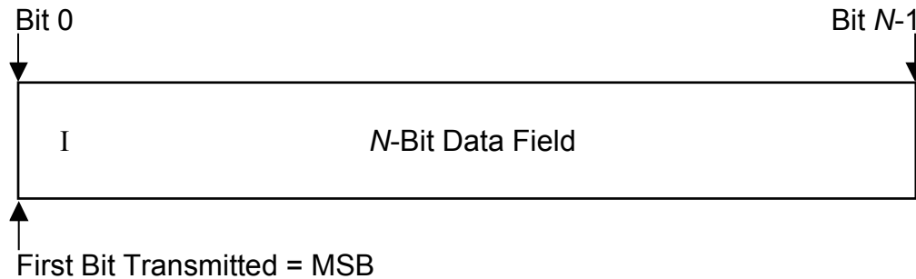
Figure 2.4.23-2: Bit Numbering Convention
