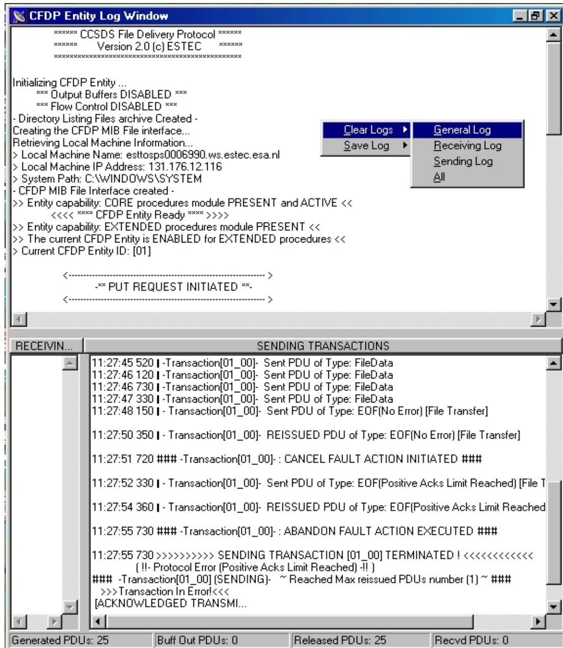
Figure 8-10: CFDP Component's Log Window
